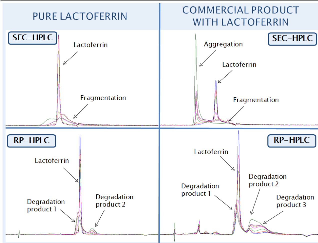
Figure 1: Chromatograms of pure Lf and commercial product with Lf stored for 0 min, 15 min, 30 min, 60 min, 120 min, 240 min, and 24 h at 60 °C.
