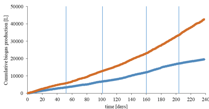
Figure 2: Cumulative biogas production in digesters R1 and R2. Vertical lines represent the periods of adding the same amount of acid whey to the digester R2 (1 L, 2 L, 3 L, 4 L and 5,5 L).
