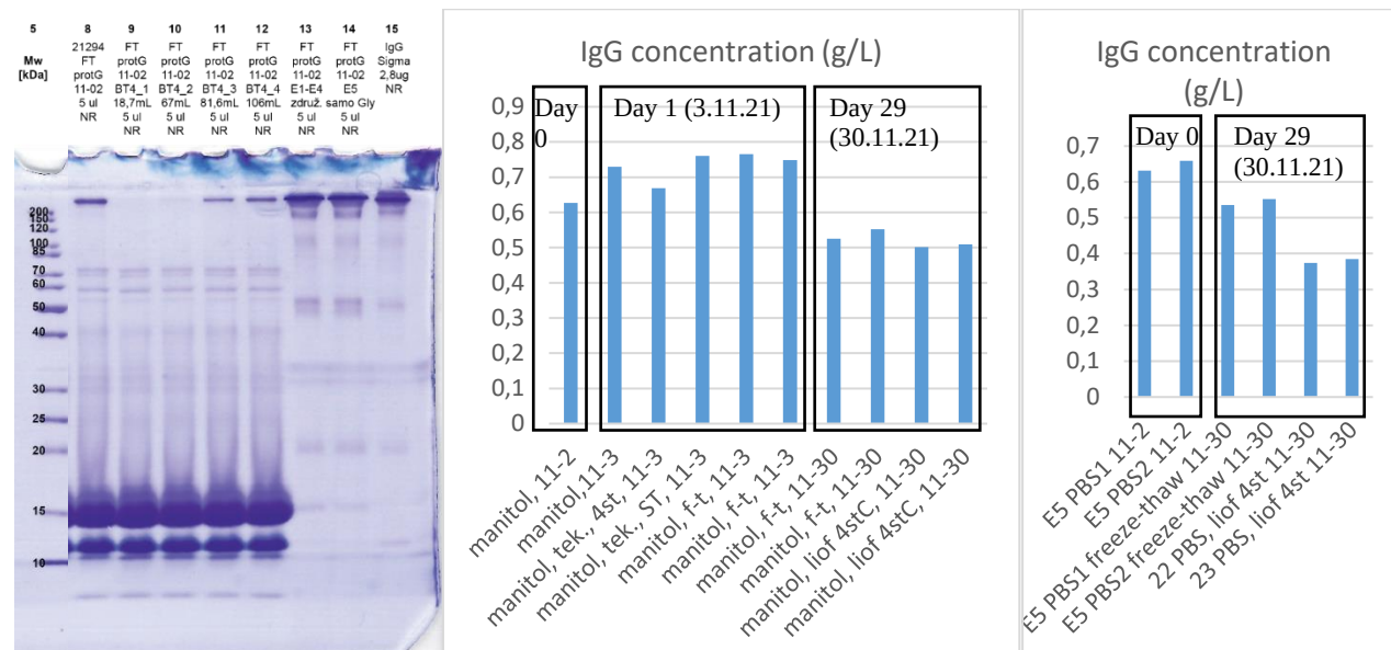
Figure 1: Left: Analysis of input acid whey (FT), unbound fractions, elutions, and commercial IgG (Sigma-Aldrich) by SDS-PAGE. Middle: IgG concentration in manitol fractions. Right: IgG concentration in manitol-free fractions.
