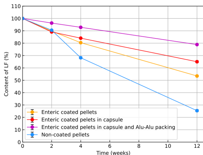
Figure 2: Stability of LF in pellets at accelerated storage conditions.
